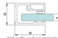
Wall profile on fixed elements
