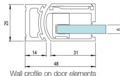
Wall profile on door elements
